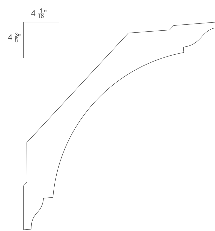
1 \frac{5}{16} " x 6" JM3381
