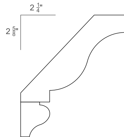
13/16" x 3-7/16" (overall) 3/4" x 2 1/16" (crown) 5/8" x 3/4" JM3411
