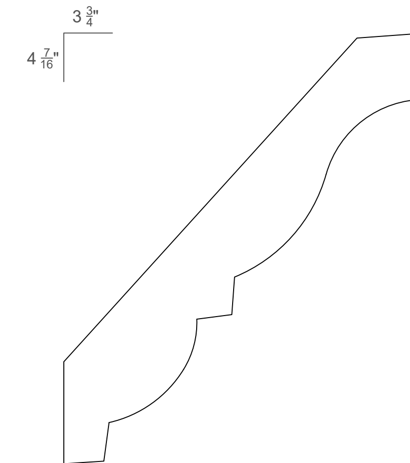
1" X 5 \frac{3}{4} " JM4601
