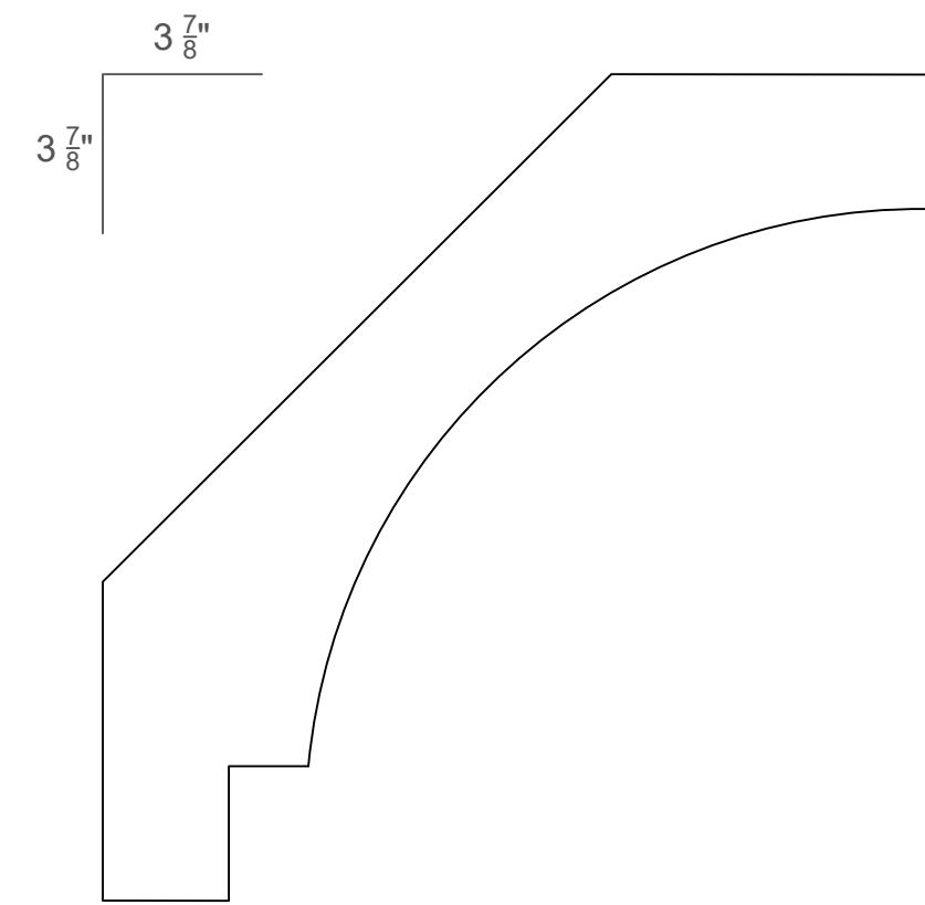
1 \frac{1}{2} " X 5 \frac{1}{2} " JM4354
