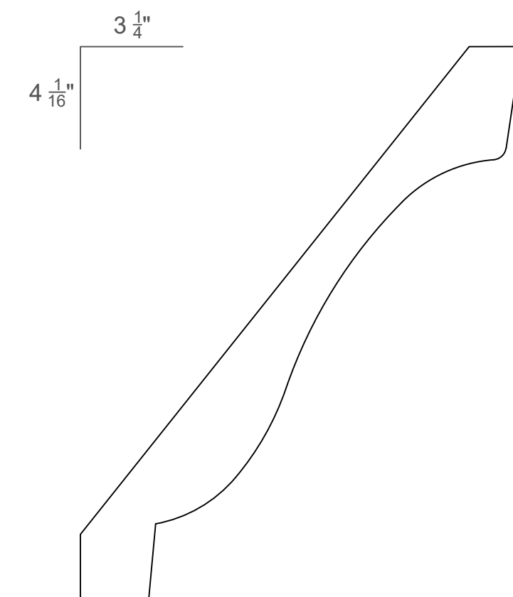
1 \frac{1}{16} " X 5 \frac{3}{16} " JM4376
