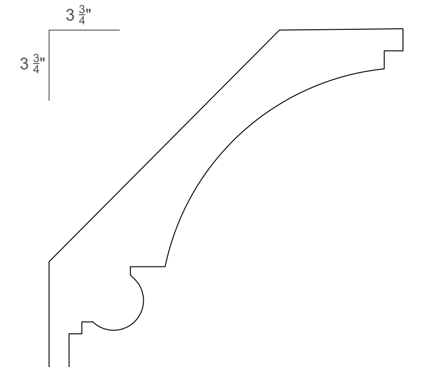
1 \frac{1}{8} " X 5 \frac{5}{16} " JM4317
