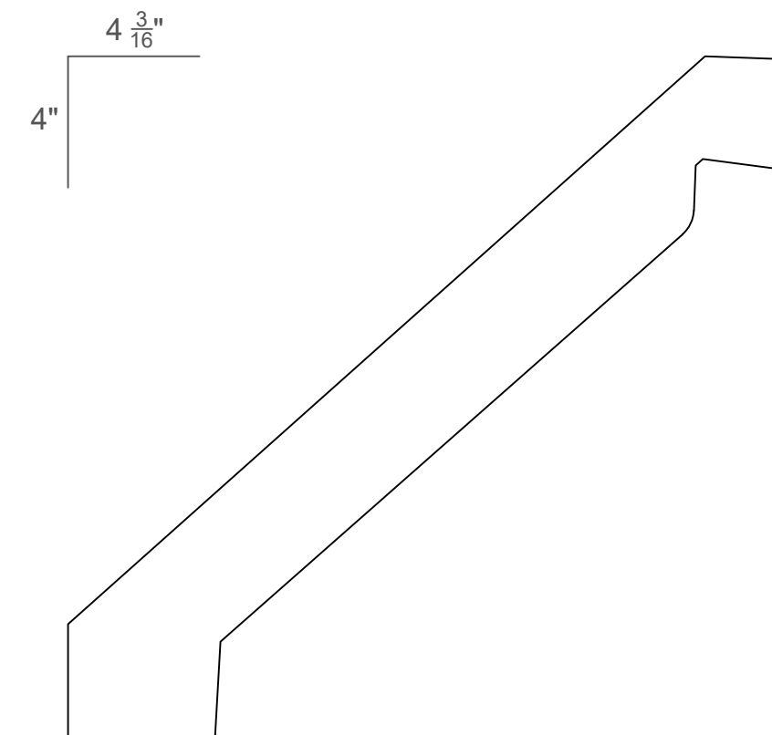
1 \frac{1}{16} " X 5 \frac{3}{4} " JM4049
