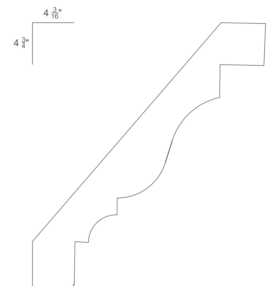
1 \frac{1}{16} " x 6 \frac{5}{16} " JM4367
