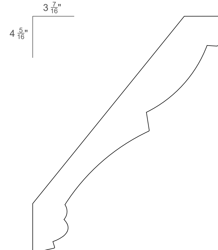
1 \frac{3}{16} " X 5 \frac{1}{2} " JM4129
