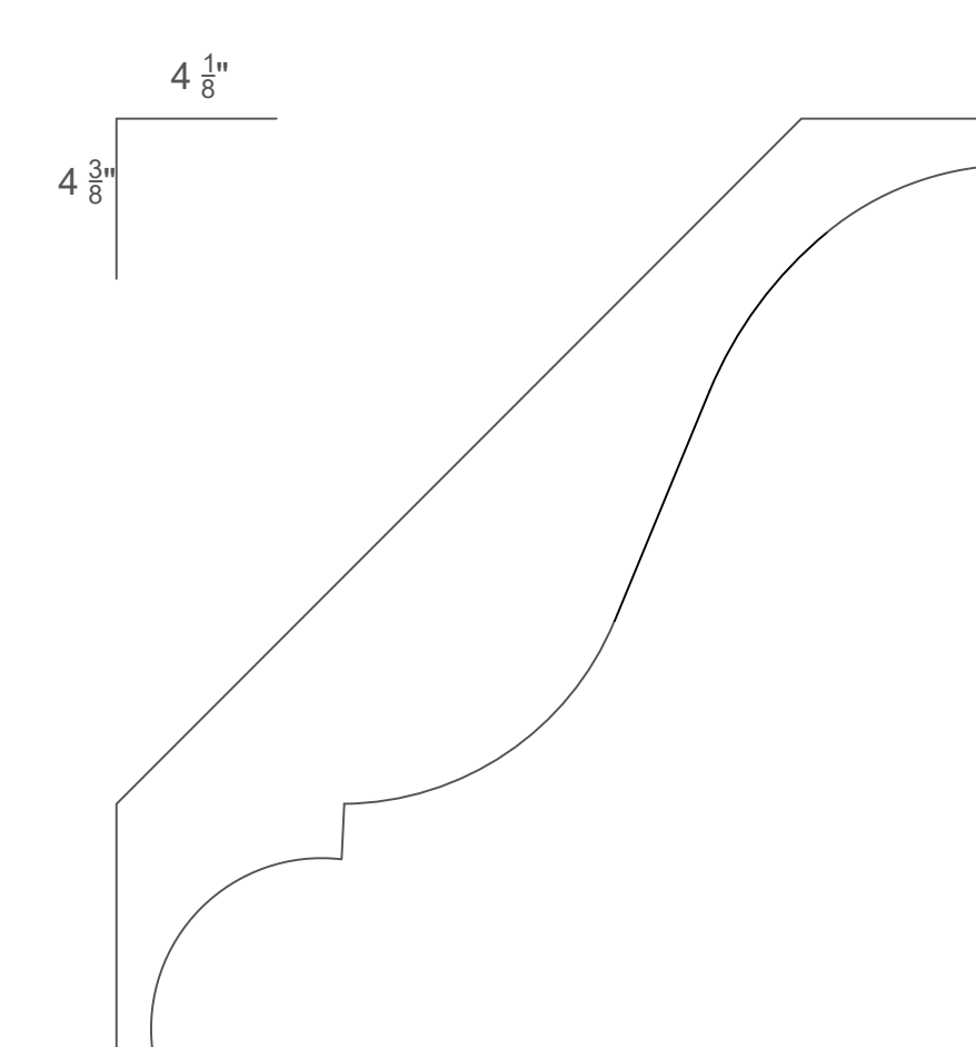
1 \frac{1}{8} " x 6" JM3257
