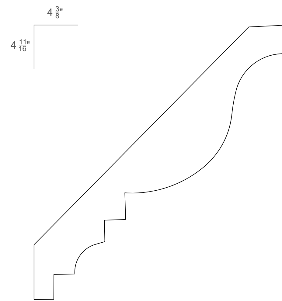
1 \frac{1}{8} " x 6 \frac{7}{16} " JM3263
