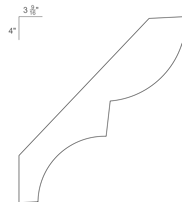
1 \frac{1}{16} " X 5 \frac{3}{4} " JM4557
