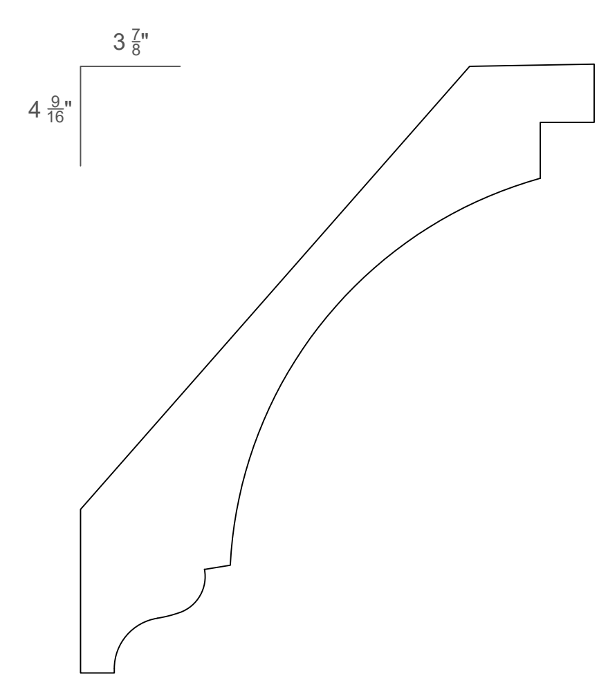
1 \frac{1}{8} " x 6" JM3798
